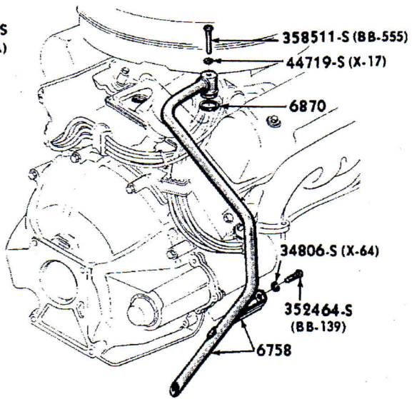
8 CYL. 292 ENGINE STANDARD VENTILATION
